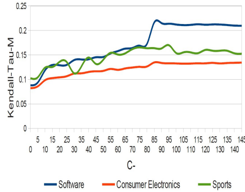
Fig. 1. Variation of Kendall-Tau-M ( \tau_m ) on different Amazon domains with parameter C^- variation (using model M_{\text{Yelp}} trained in Yelp and tested in Amazon).
